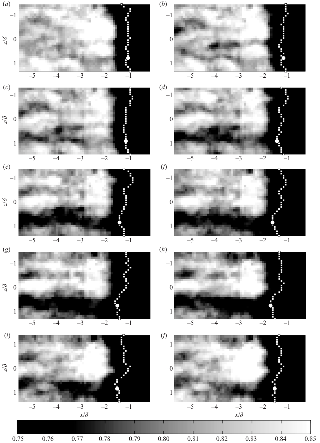
FIGURE 10. A sequence of running-averaged streamwise velocity contours at y/\delta = 0.2 . Subsequent plots are separated by 166\mu\text{s} . The vector fields are filtered by computing a six-frame running average. The streamwise velocity is normalized by the free stream velocity ( U_\infty ). Flow is left to right.
